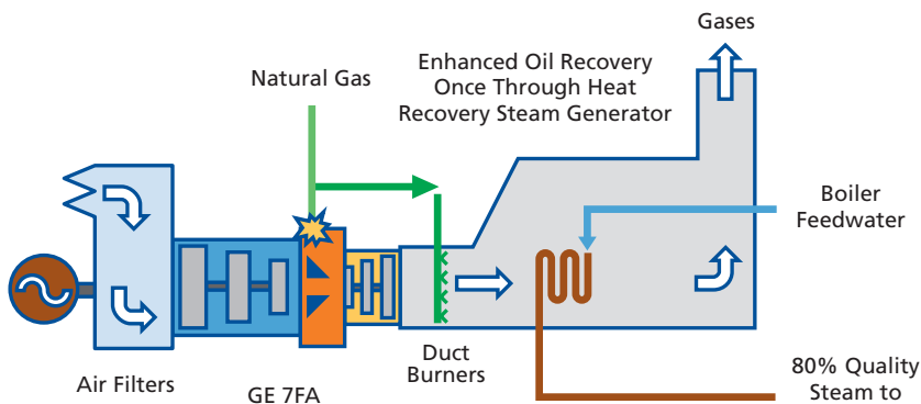
MacKay River plant schematic
